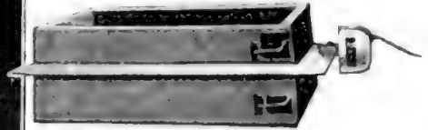
Below: An electric vibrator attached to a pattern-plate to take the place of hand rapping
